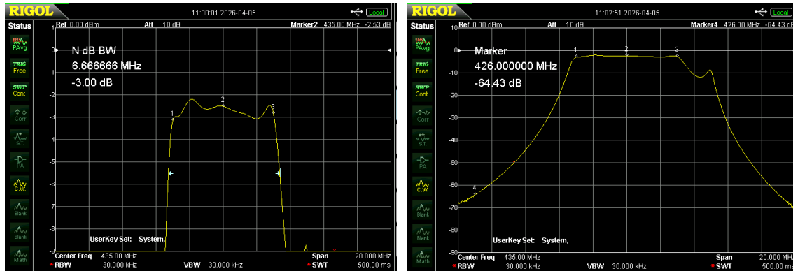
Fig. 11 Receiver's Band-Pass Filter S21 frequency response. center freq. = 435 MHz, left is pass-band response 1dB/div & 2 MHz/div right is stop-band response 10dB/div & 2 MHz/div. Insertion loss = -2.5dB -3dB BW = 6.7 MHz
