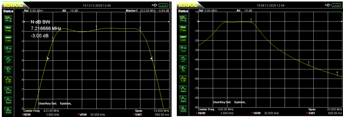
Fig. 9 S21 swept frequency response for Ch 57, transmitter band-pass filter. One UHF-TV-3P filter. left pass-band response, center freq. = 423MHz, 1dB/div & 1MHz/div. Insertion loss = -0.9dB, -3dB BW = 7.2 MHz. right stop-band response, center freq = 430 MHz, 10dB/div & 3MHz/div
