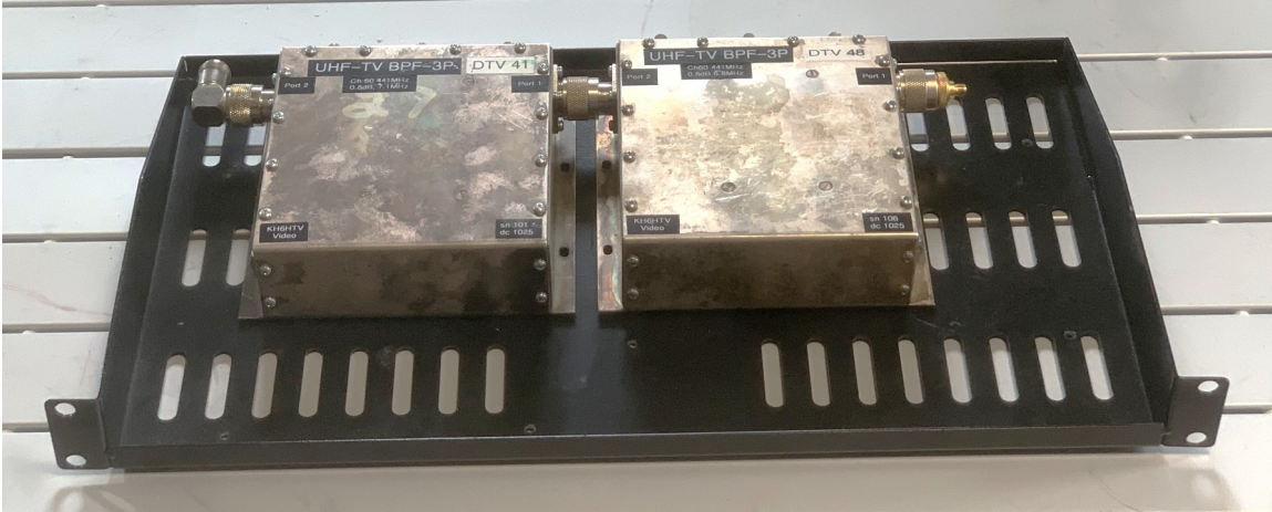
Fig. 7 1U relay rack tray holding the two UHF-TV-3P, Ch 59 receive band-pass filters
