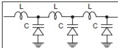
Fig. 1 Non-Linear Transmission Line Schematic
