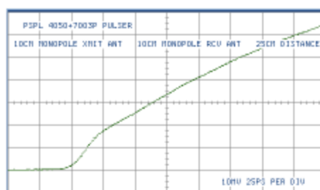
Fig. 15 Transmission between a pair of identical 10 cm monopole antennas.
