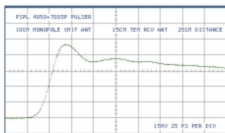
Fig. 13 Transmission from monopole to TEM
