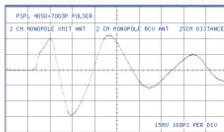
Fig. 17 Transmission between a pair of identical 2 cm monopole antennas. 100 ps/div
