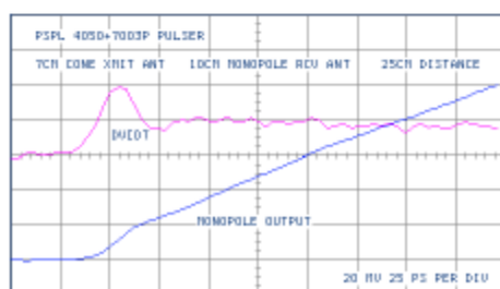
Fig. 14 Transmission from conical to monopole Lower trace rcv. ant. output. Upper trace is dV/dt
